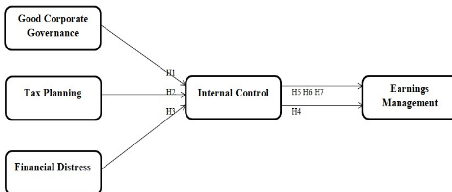
Figure 1 Framework
